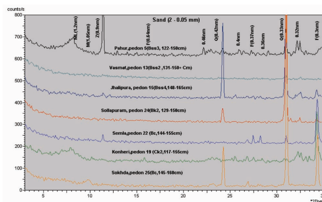
Figure 7. Representative XRD patterns of sand fractions showing presence of zeolites in Vertisols of different climatic regions. ML, Mica-vermiculite; M, mica; Z, Zeolite; Q, quartz; F, Feldspars.
