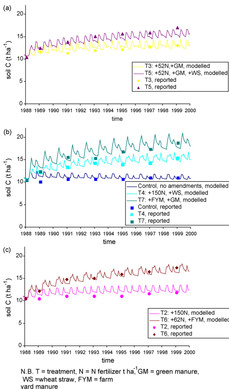
Fig. 2. (a–c) Modelled and measured soil carbon over time for seven management regimes included in the long-term fertilizer trials (Nos. 14 and 15) at Ludhiana, Punjab, India.
