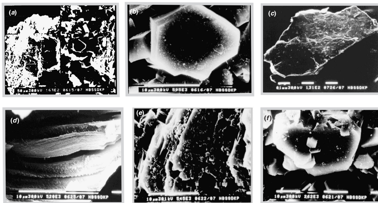
Fig. 3. Representative SEM photographs of sand-sized fractions showing (a) a cluster of hexagonal and rod-shaped gibbsites developed on feldspars (Bt2 layer of Pedon 3), (b) well-developed hexagonal prisms of individual gibbsite (Bt2 layer of Pedon 3), (c) biotite grain that escaped tropical weathering, (d) initiation of layer separation in biotite particle effecting the formation of vermiculite, (e) highly weathered feldspar grains showing the dissolution and etch pits with gibbsite crystals, (f) same as (e) at higher magnification.
