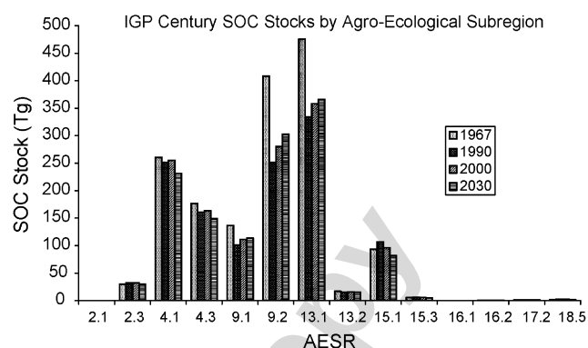
Fig. 5. SOC stock for 1967, 1990, 2000 and 2030 according to the Century module of the GEFSOC Modelling System by agro-ecological sub-regions in the Indian IGP.
