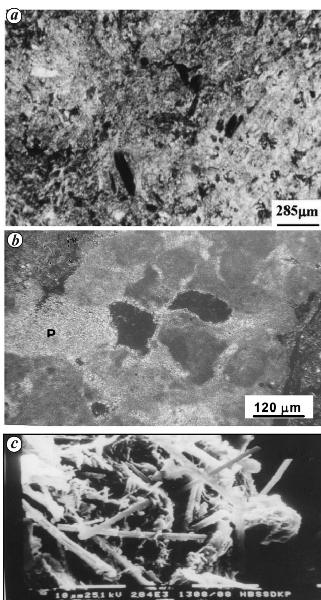
Figure 1. Representative photomicrographs of pedogenic \text{CaCO}_3 . a , Soils of the IGP (Natrustalfs); b , Vertisols of central India; c , Ferruginous soils of southern India (Alfisol) (adapted from Pal et al. 25 ).
