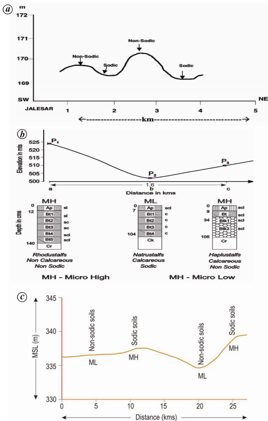
Figure 3. a , NE-SW profile in Ganga-Yamuna interfluvium of the IGP showing non-sodic soils on MH and sodic soils on ML sites. b , Schematic diagram of the landscape representing the unique role of micro topography in the formation of non-sodic and sodic RF soils at MH and ML positions. c , Juxtaposition of the occurrence of sodic and non-sodic soils (Vertisols) on MH and ML positions in black soils region (adapted from Pal et al. 25 ).
